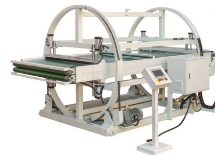
HY-TF 圆柱翻板机 HY-TF Panel turning machine
